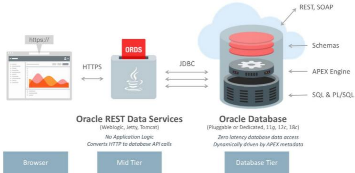
Figure 1. Oracle APEX Architecture
